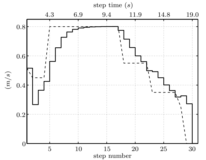
Fig. 3. Command (dashed) versus actual (solid) average walking rate (Note: the sloped portions of the command curve correspond to transition controllers, and average walking rate is computed at the end of each step).
