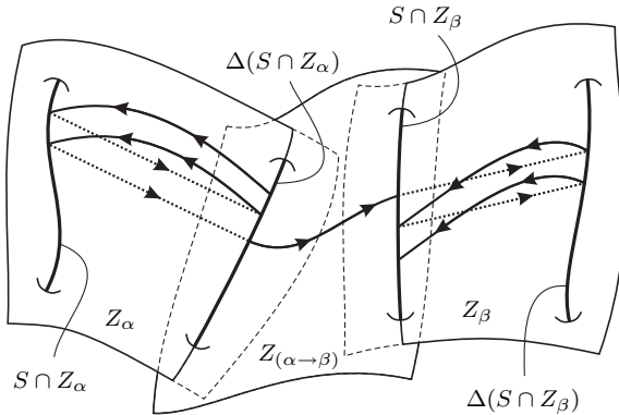
Fig. 2. Abstraction of the composition of two controllers \Gamma_\alpha and \Gamma_\beta via transition controller \Gamma_{(\alpha \rightarrow \beta)} . Under the action of \Gamma_\alpha the dynamics evolve on Z_\alpha . Switching to \Gamma_{(\alpha \rightarrow \beta)} when the state enters \Delta(S \cap Z_\alpha) causes the dynamics to evolve along Z_{(\alpha \rightarrow \beta)} to S \cap Z_\beta . Switching to \Gamma_\beta when the state enters S \cap Z_\beta causes the dynamics to evolve on Z_\beta .
