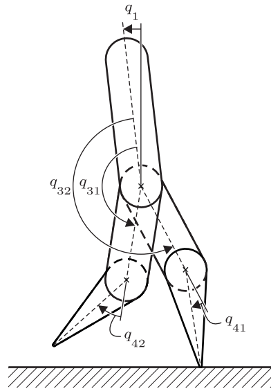
Fig. 1. Schematic of five-link model studied.
